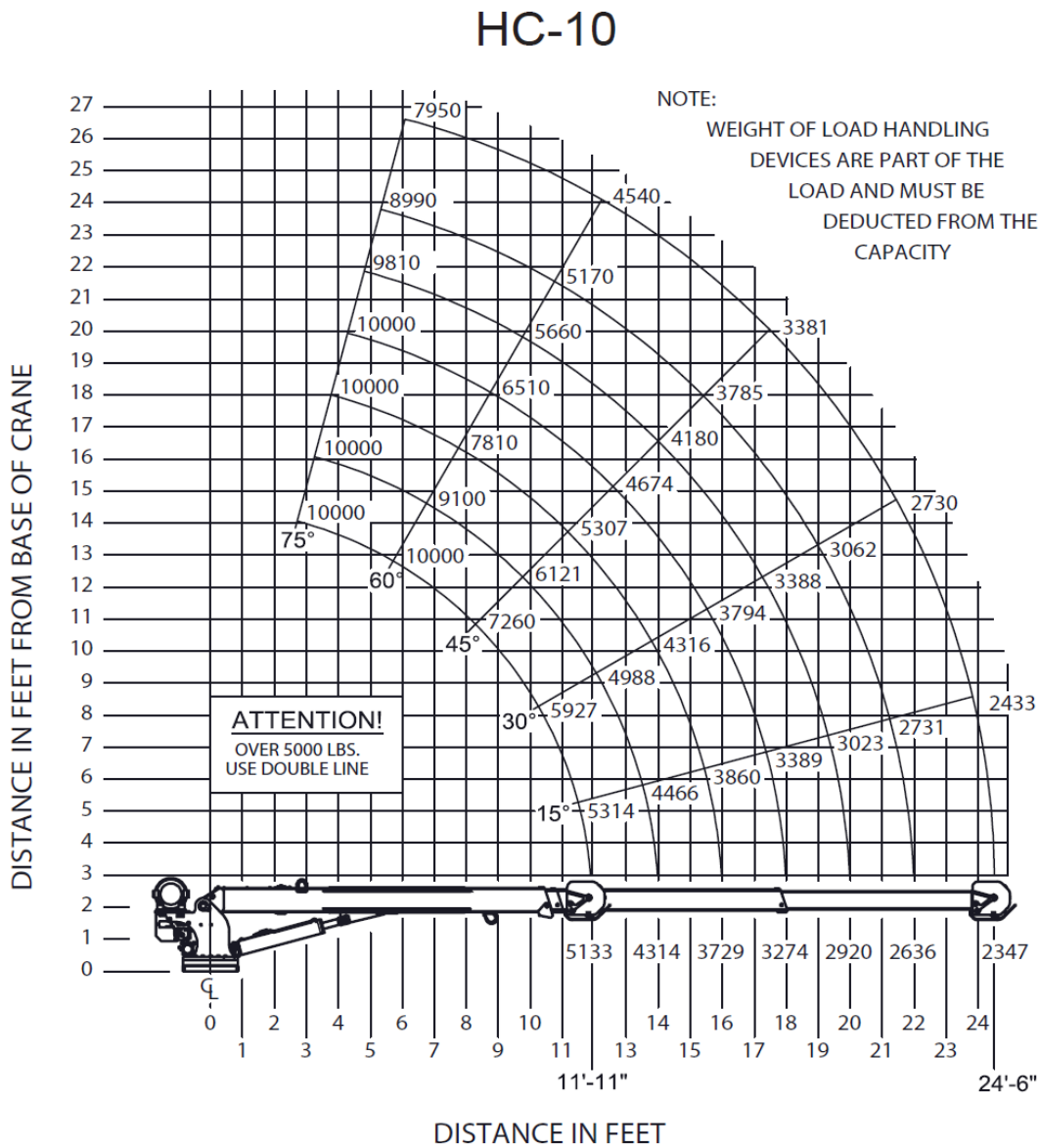
Figure 1: HC-10 Load Chart
