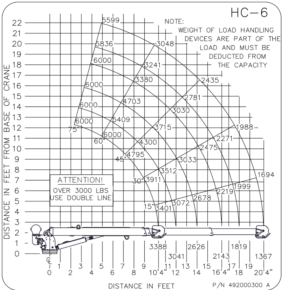
Figure 1: HC-6 Load Chart
