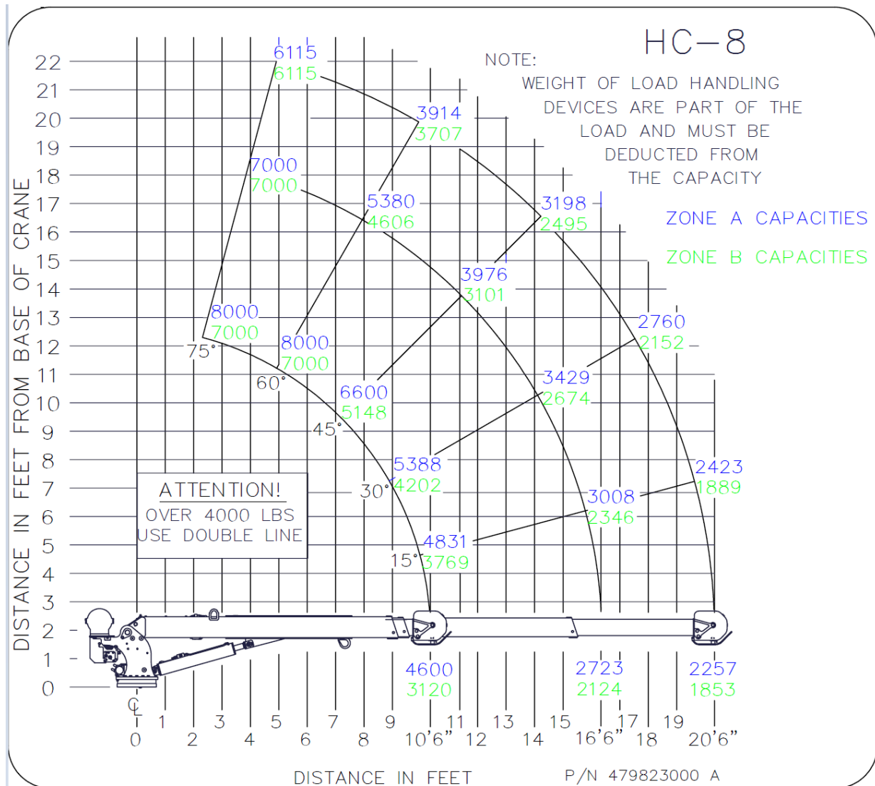
Figure 1: HC-8 Load Chart
